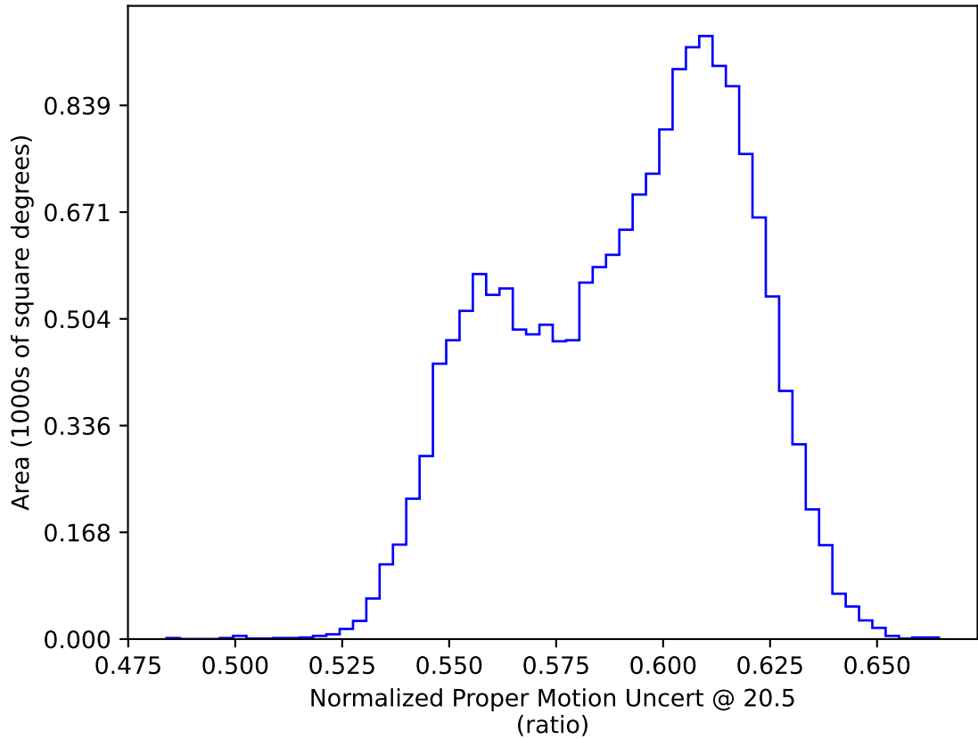
ddf_acor_sf20_lsf0_lsr0_v3.4_10yrs WFD: Normalized Proper Motion Uncert @ 20.5
