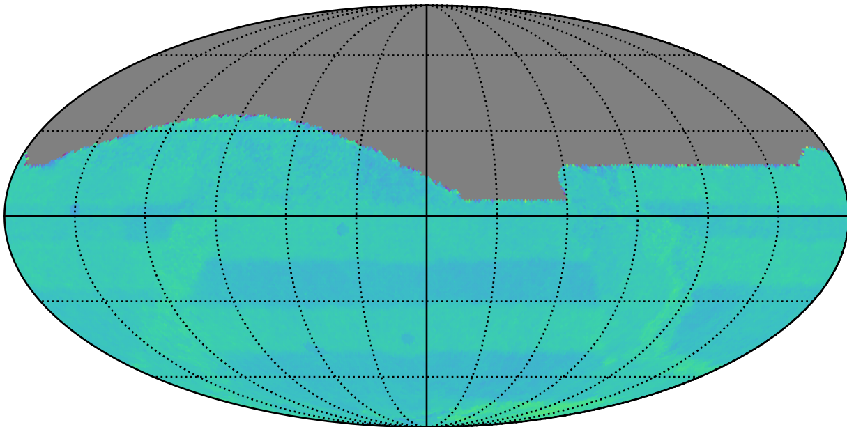
ddf_acor_sf20_lsf0_lsr0_v3.4_10yrs All sky: Normalized Proper Motion Uncert @ 20.5
