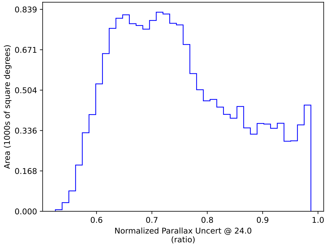
ddf_acor_sf20_ls0_lsr0_v3.4_10yrs WFD: Normalized Parallax Uncert @ 24.0
