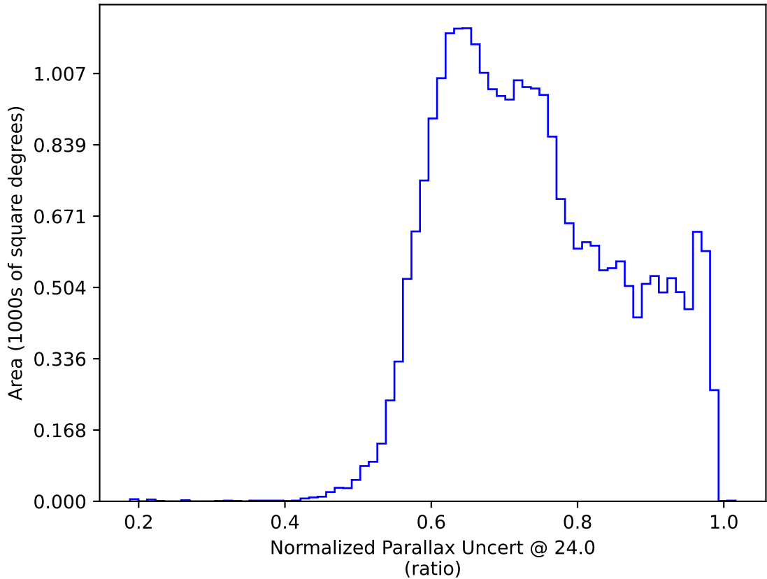
ddf_acor_sf20_lsf0_lsr0_v3.4_10yrs All sky: Normalized Parallax Uncert @ 24.0
