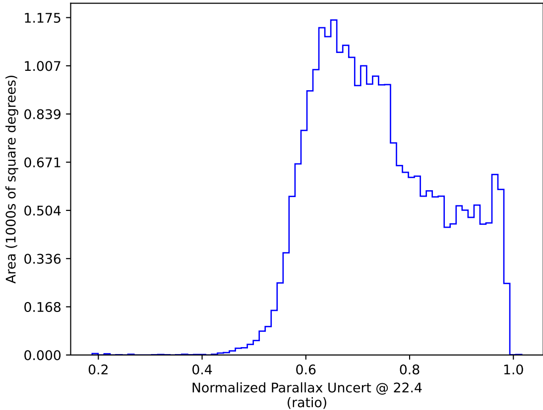
ddf_acor_sf20_lsf0_lsr0_v3.4_10yrs All sky: Normalized Parallax Uncert @ 22.4
