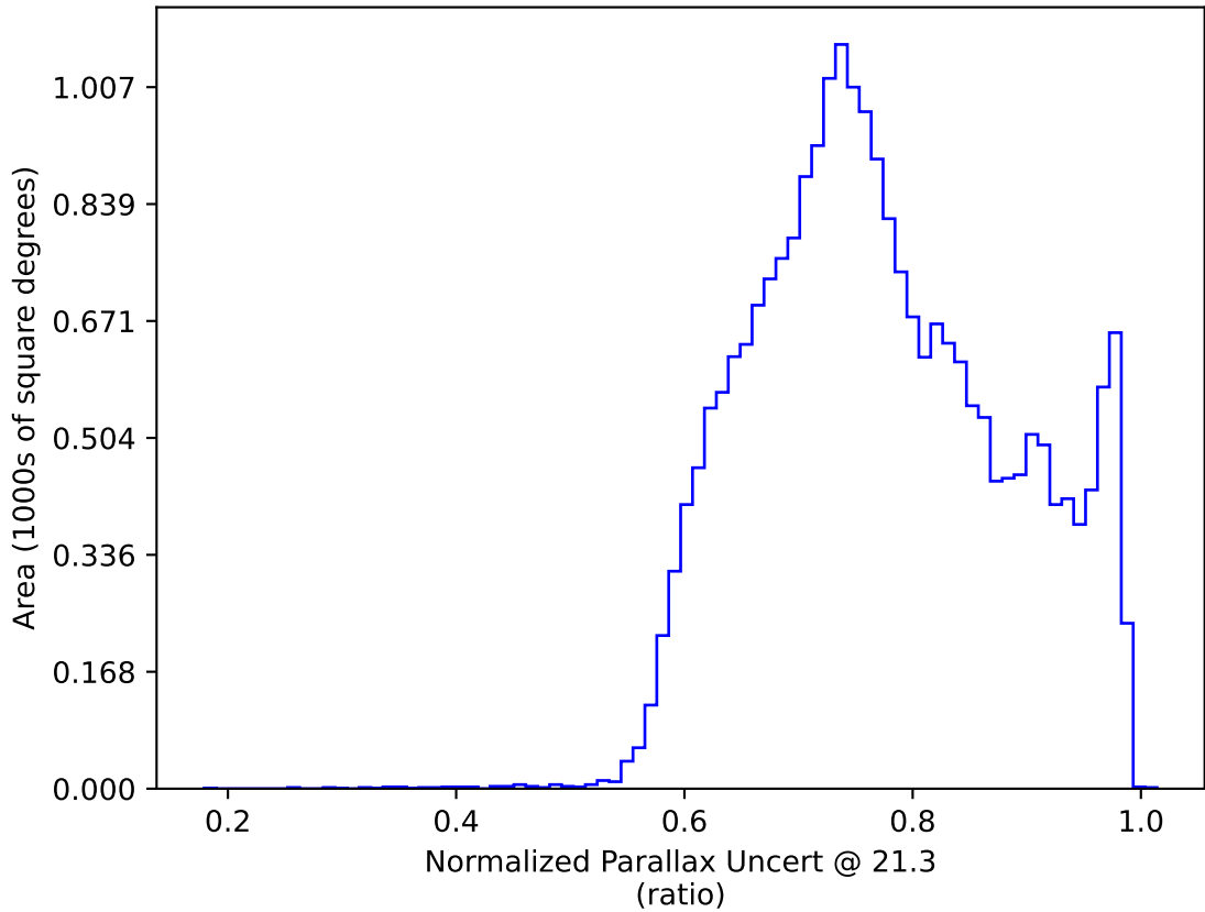
ddf_acor_sf20_lsf0_lsr0_v3.4_10yrs All sky y band only: Normalized Parallax Uncert @ 21.3
