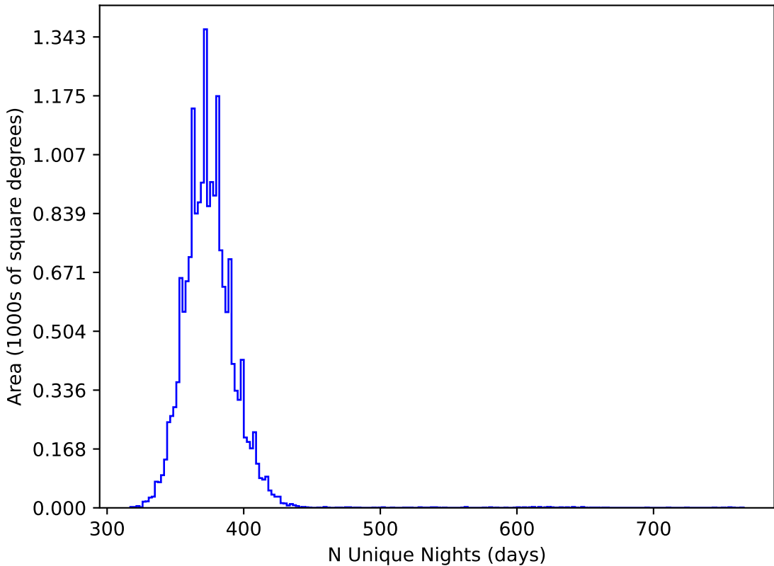
ddf_acor_sf20_ls0_lsr0_v3.4_10yrs WFD all bands: N Unique Nights
