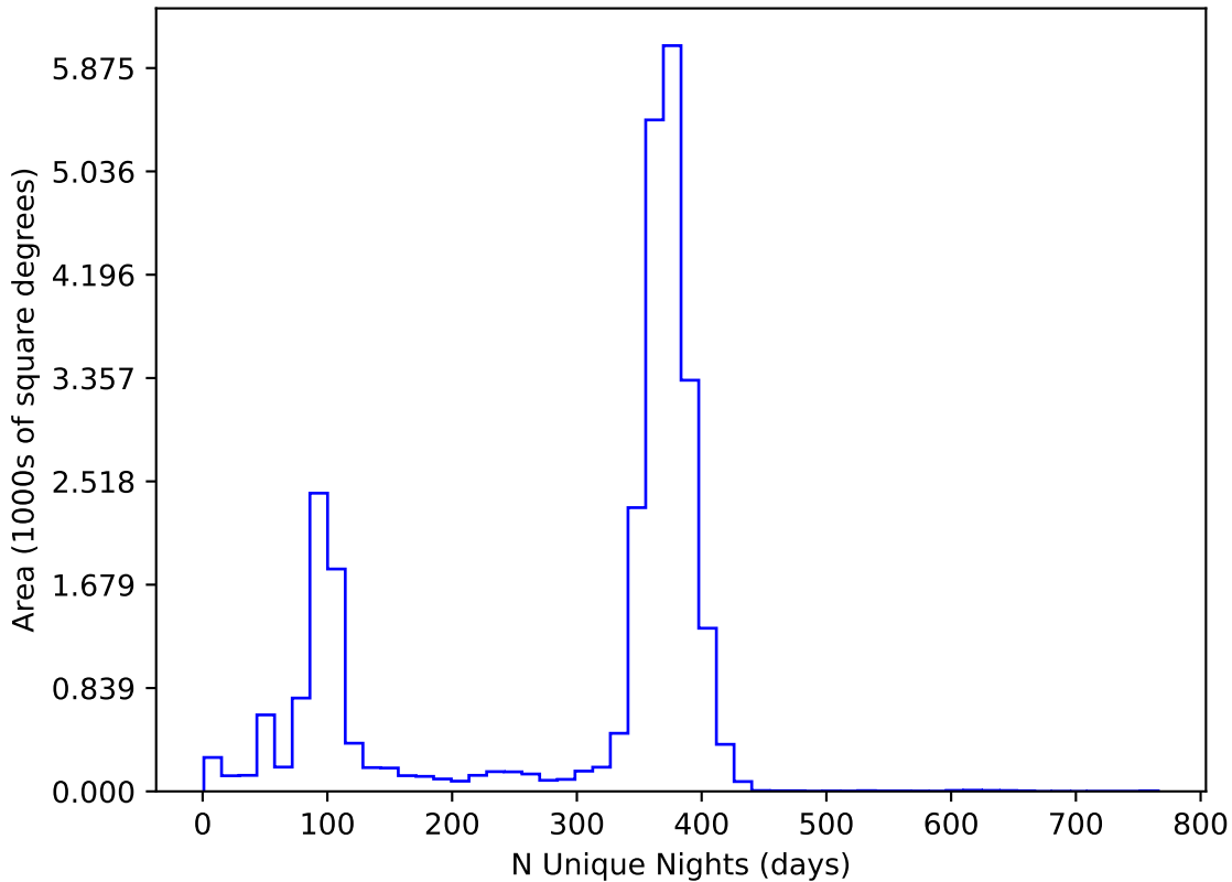
ddf_acor_sf20_lsf0_lsr0_v3.4_10yrs All sky all bands: N Unique Nights
