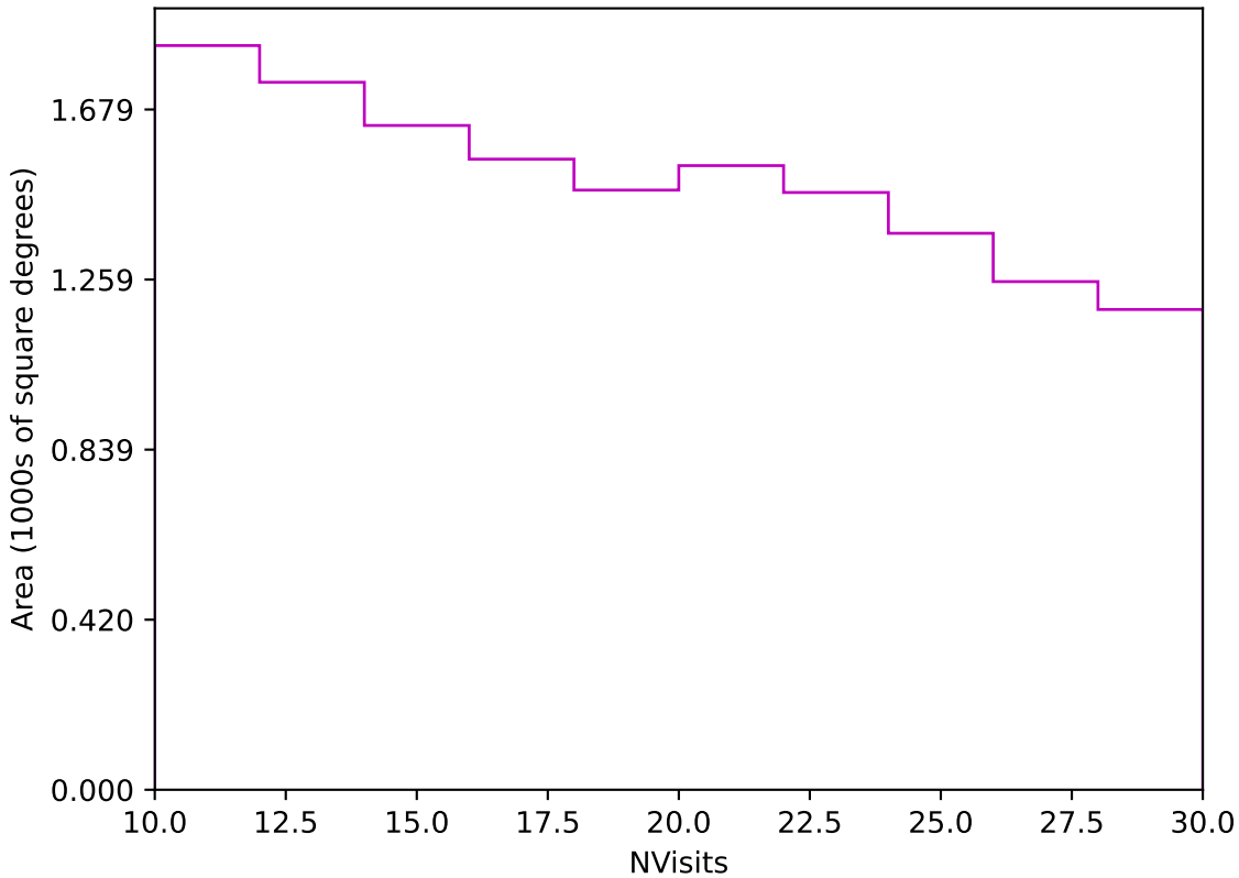
ddf_acor_sf20_lsf0_lsr0_v3.4_10yrs Yr 3-4 z band: NVisits
