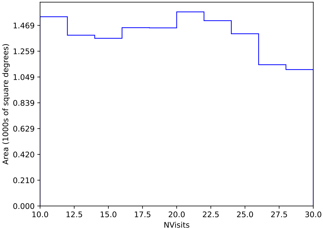
ddf_acor_sf20_lsf0_lsr0_v3.4_10yrs Yr 3-4 y band: NVisits
