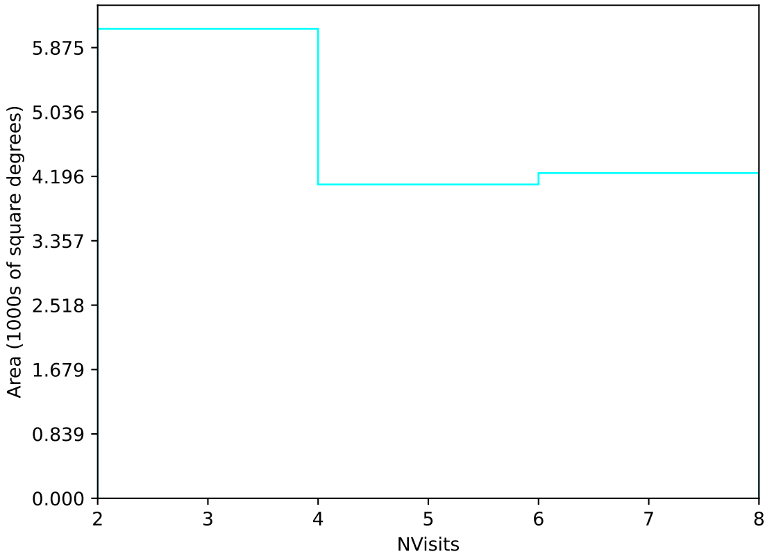
ddf_acor_sf20_lsf0_lsr0_v3.4_10yrs Yr 3-4 u band: NVisits
