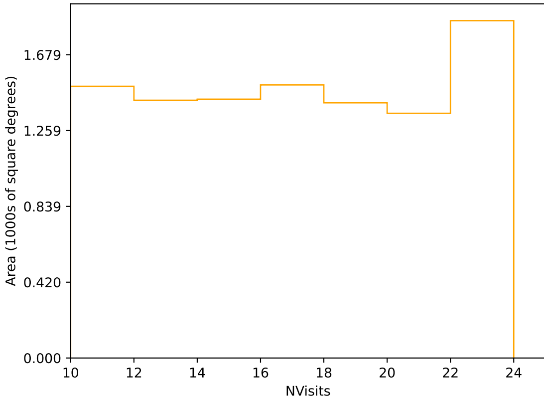
ddf_acor_sf20_lsf0_lsr0_v3.4_10yrs Yr 3-4 r band: NVisits
