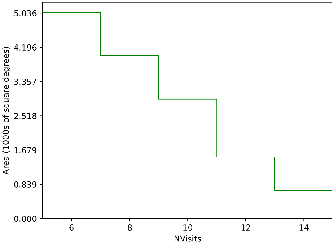
ddf_acor_sf20_lsf0_lsr0_v3.4_10yrs Yr 3-4 g band: NVisits
