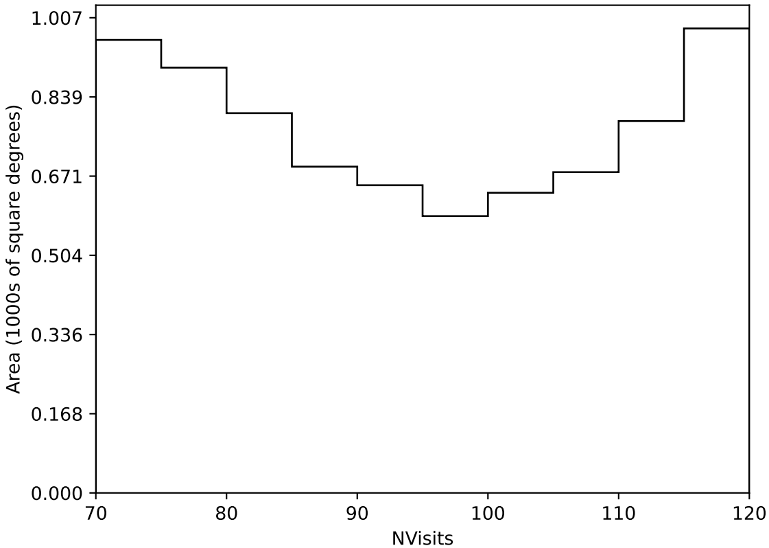
ddf_acor_sf20_lsf0_lsr0_v3.4_10yrs Yr 3-4 all bands: NVisits
