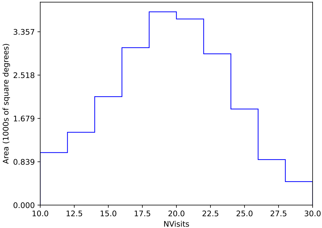
ddf_acor_sf20_lsf0_lsr0_v3.4_10yrs Yr 1 y band: NVisits
