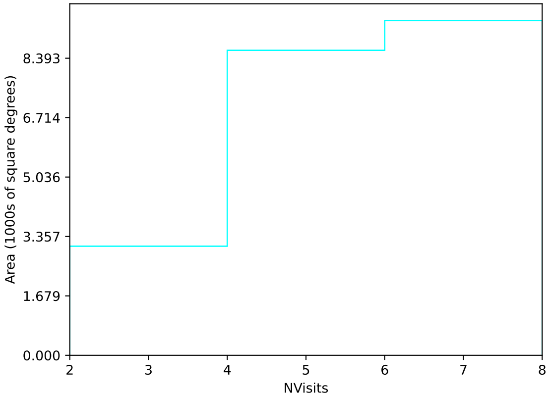
ddf_acor_sf20_lsf0_lsr0_v3.4_10yrs Yr 1 u band: NVisits
