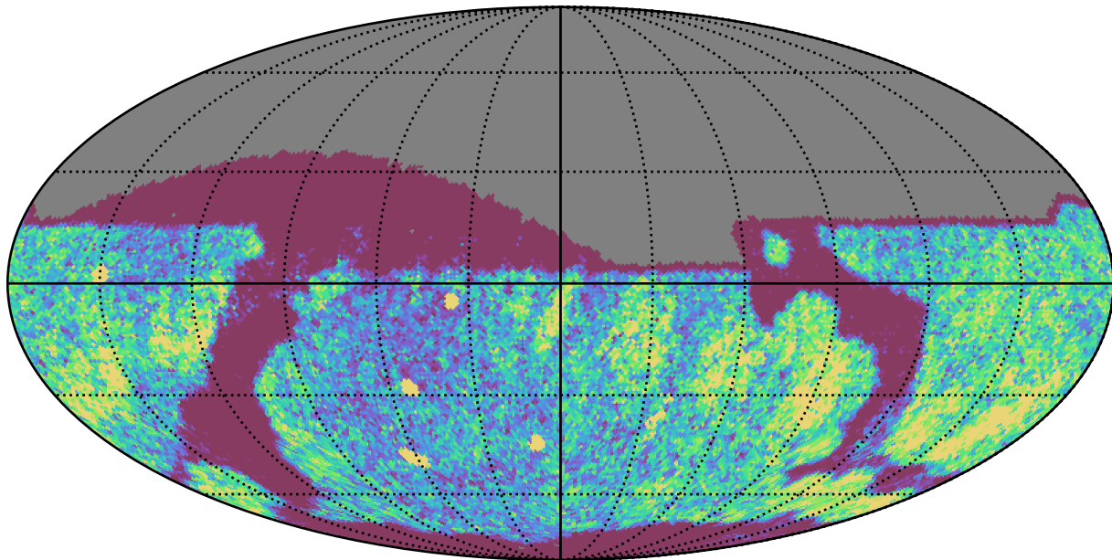
ddf_acor_sf20_lsf0_lsr0_v3.4_10yrs Yr 1 r band: NVisits
