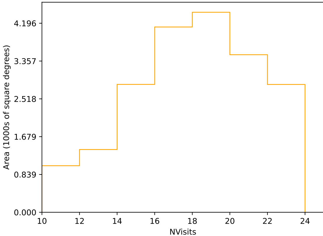
ddf_acor_sf20_lsf0_lsr0_v3.4_10yrs Yr 1 r band: NVisits
