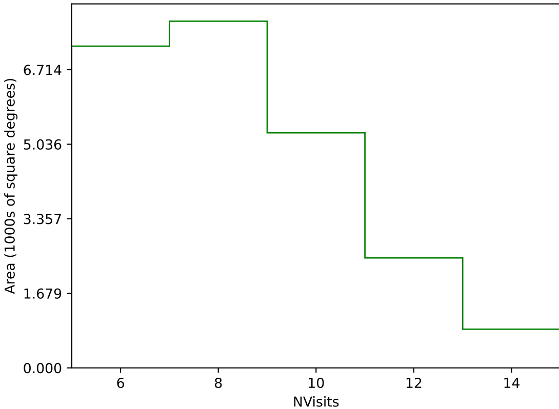
ddf_acor_sf20_lsf0_lsr0_v3.4_10yrs Yr 1 g band: NVisits
