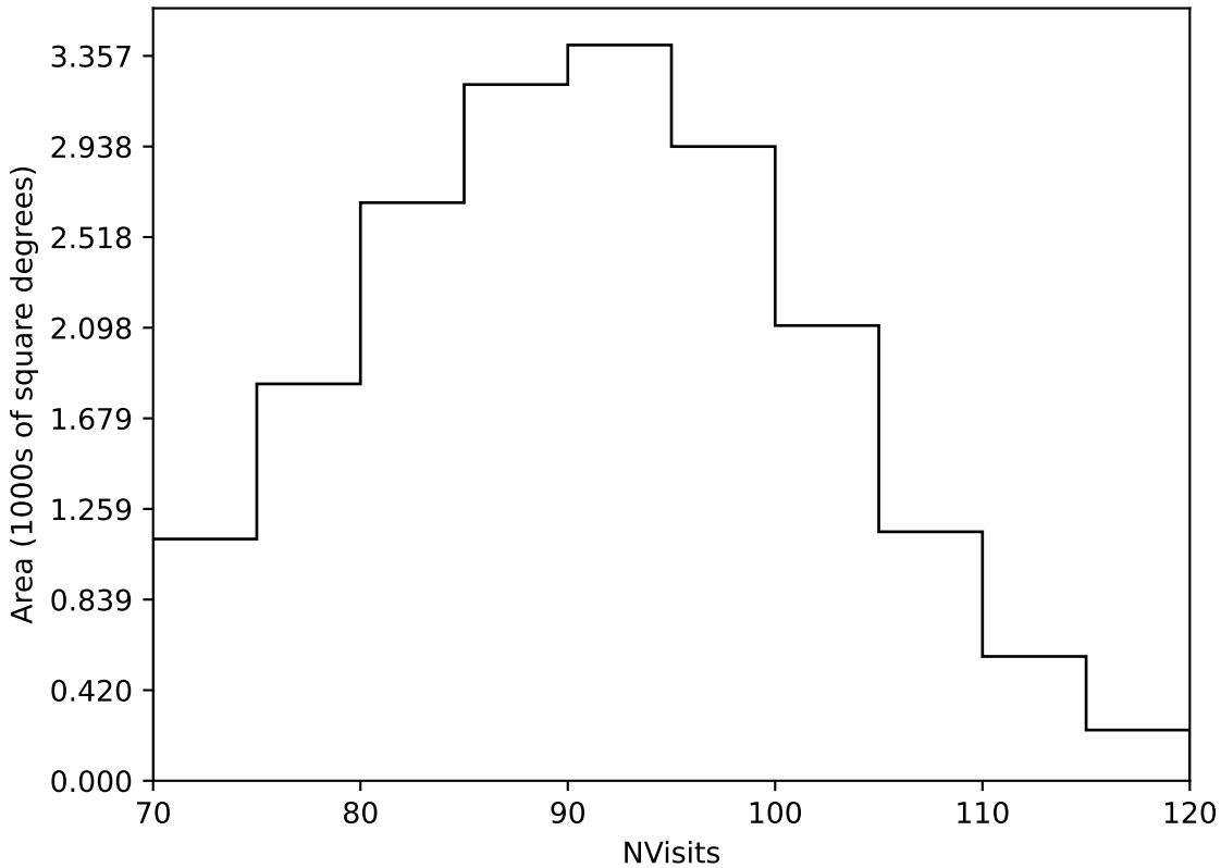
ddf_acor_sf20_lsf0_lsr0_v3.4_10yrs Yr 1 all bands: NVisits
