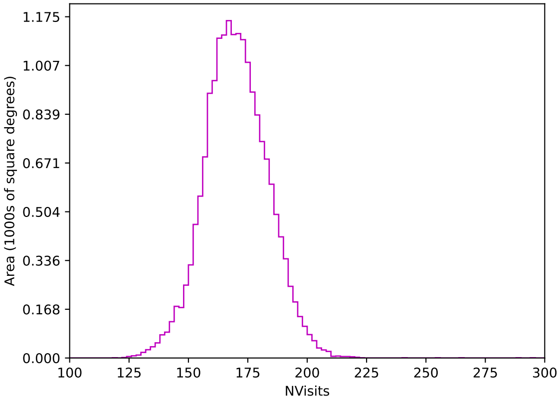
ddf_acor_sf20_lsf0_lsr0_v3.4_10yrs WFD z band: NVisits
