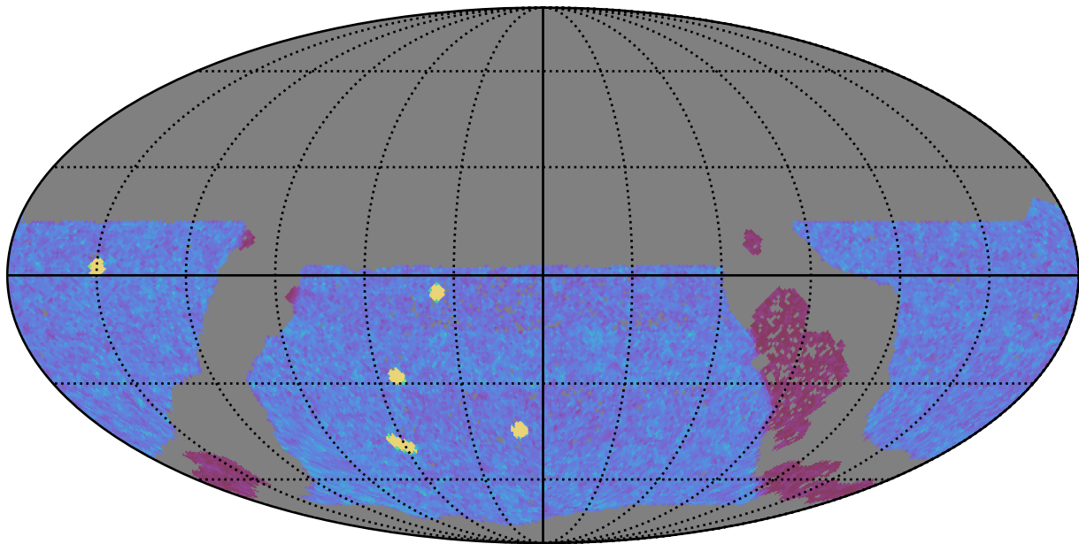
ddf_acor_sf20_lsf0_lsr0_v3.4_10yrs WFD y band: NVisits
