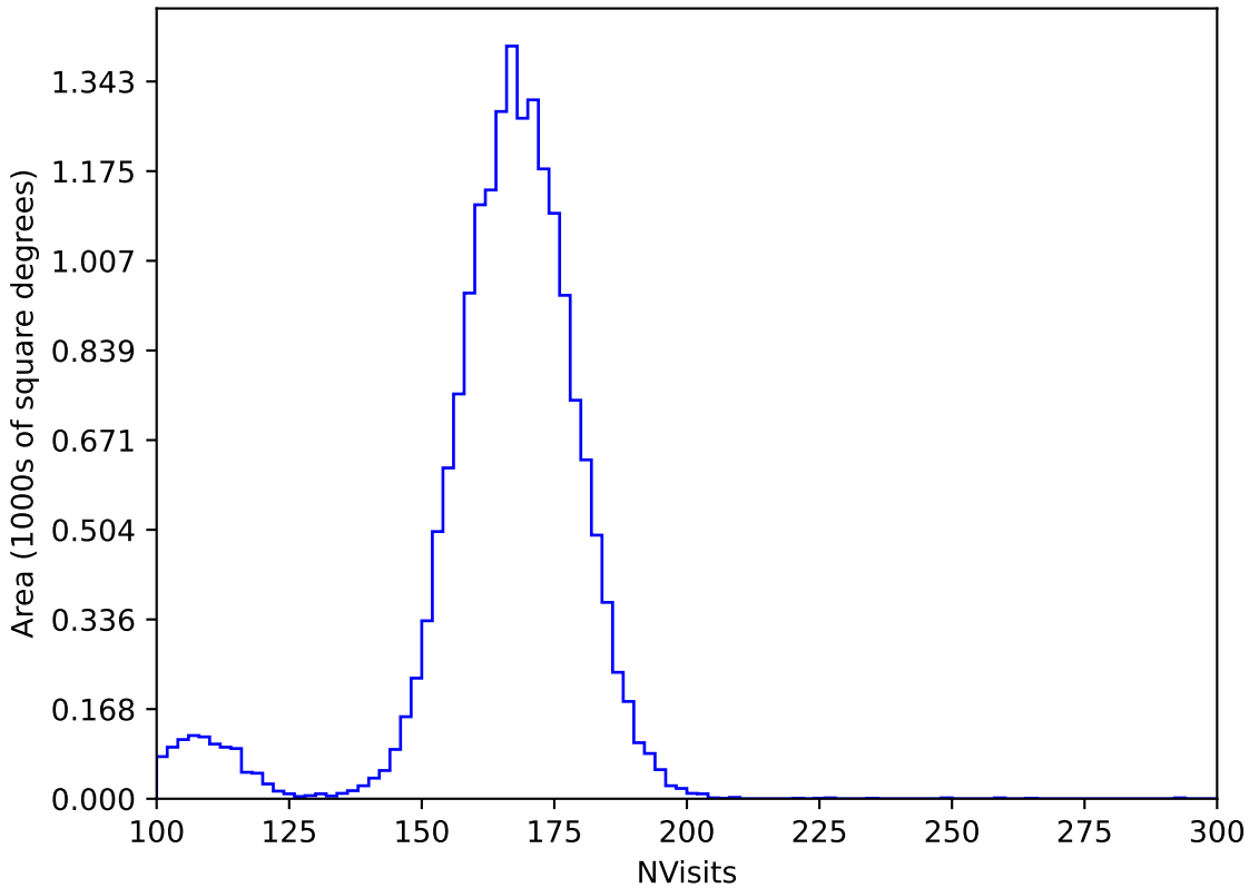
ddf_acor_sf20_ls0_lsr0_v3.4_10yrs WFD y band: NVisits
