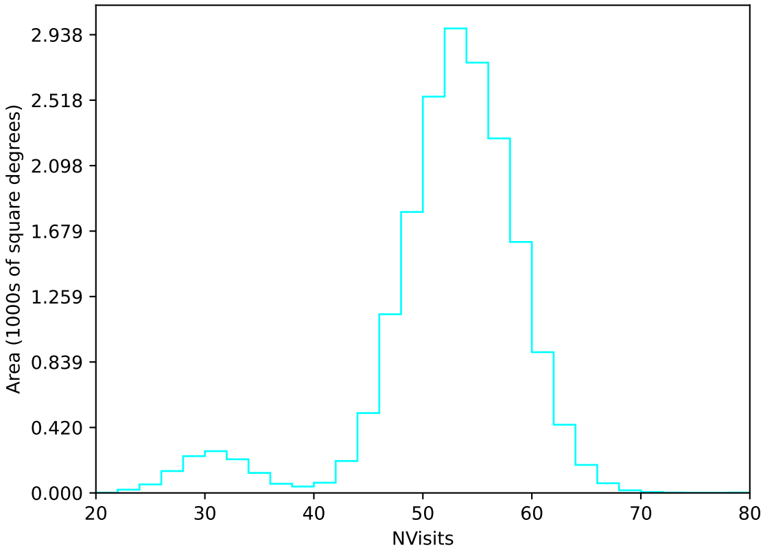
ddf_acor_sf20_lsf0_lsr0_v3.4_10yrs WFD u band: NVisits
