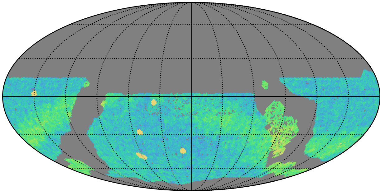
ddf_acor_sf20_lsf0_lsr0_v3.4_10yrs WFD r band: NVisits
