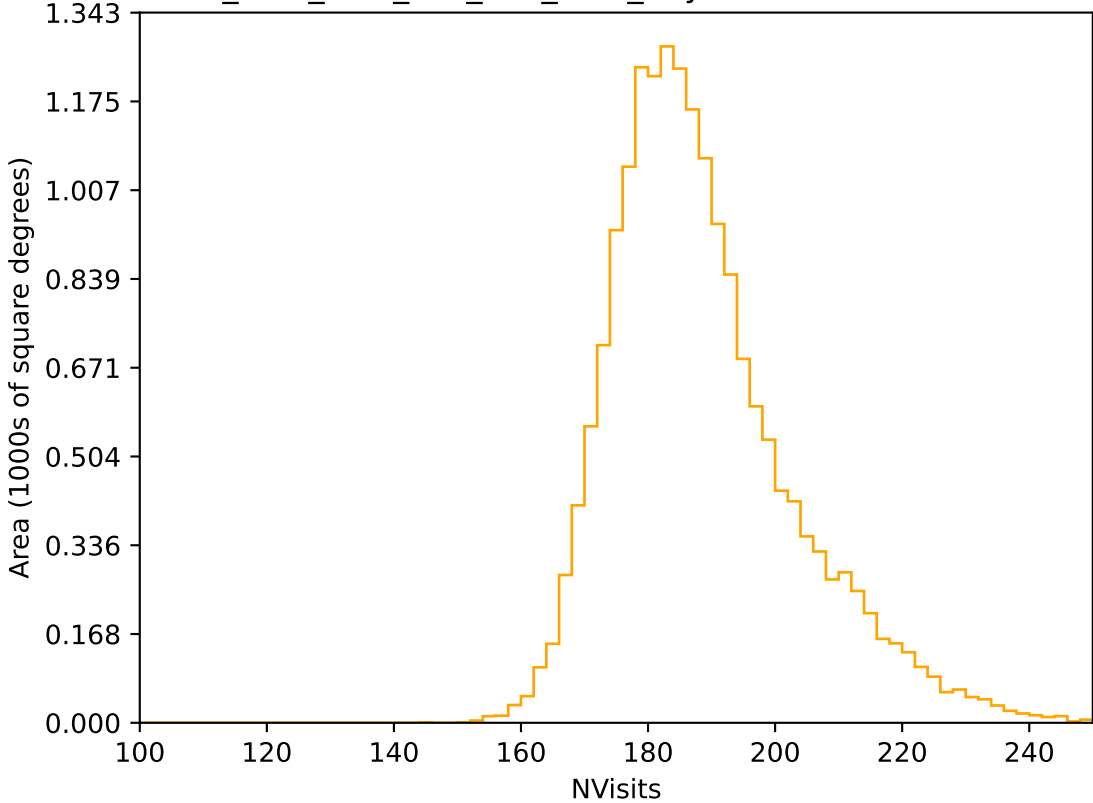
ddf_acor_sf20_lsf0_lsr0_v3.4_10yrs WFD r band: NVisits
