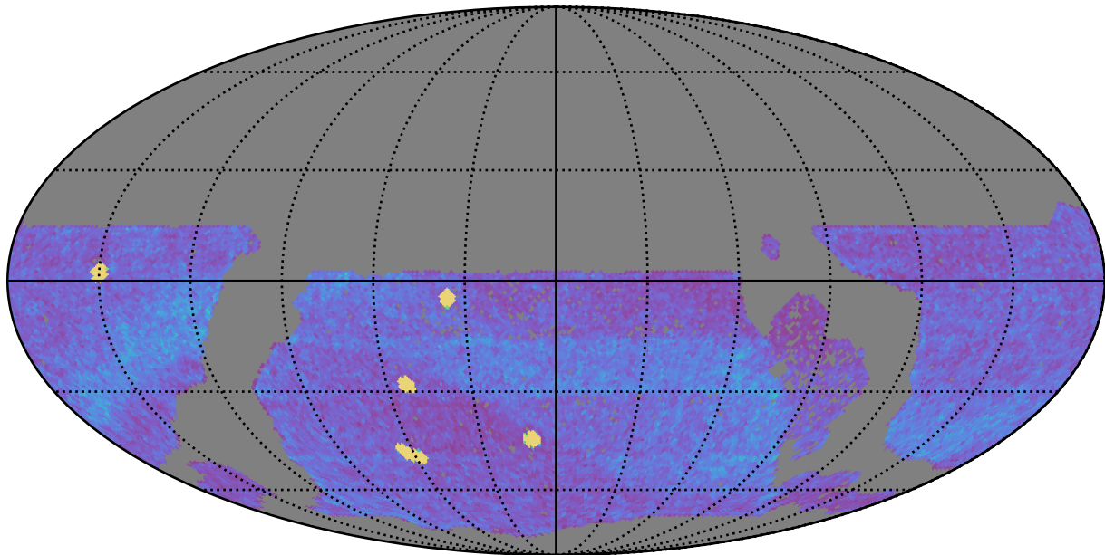
ddf_acor_sf20_lsf0_lsr0_v3.4_10yrs WFD all bands: NVisits
