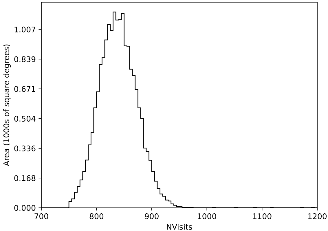
ddf_acor_sf20_lsf0_lsr0_v3.4_10yrs WFD all bands: NVisits
