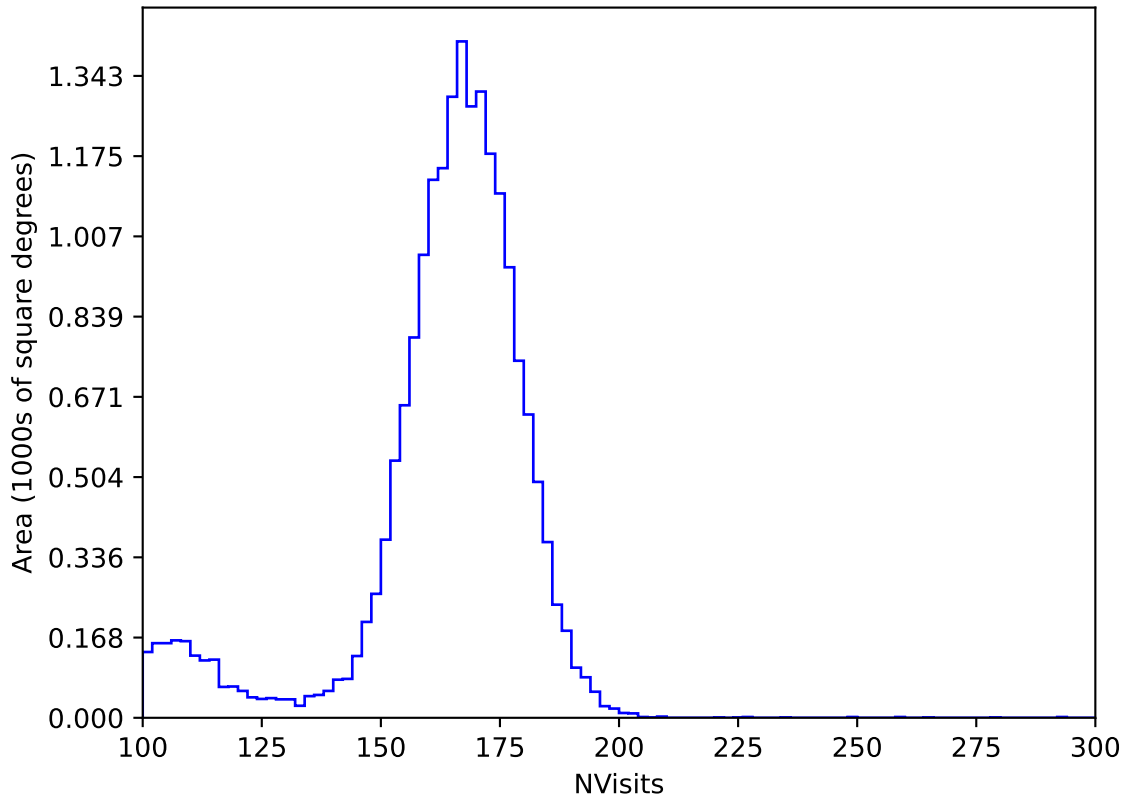
ddf_acor_sf20_lsf0_lsr0_v3.4_10yrs All sky y band: NVisits
