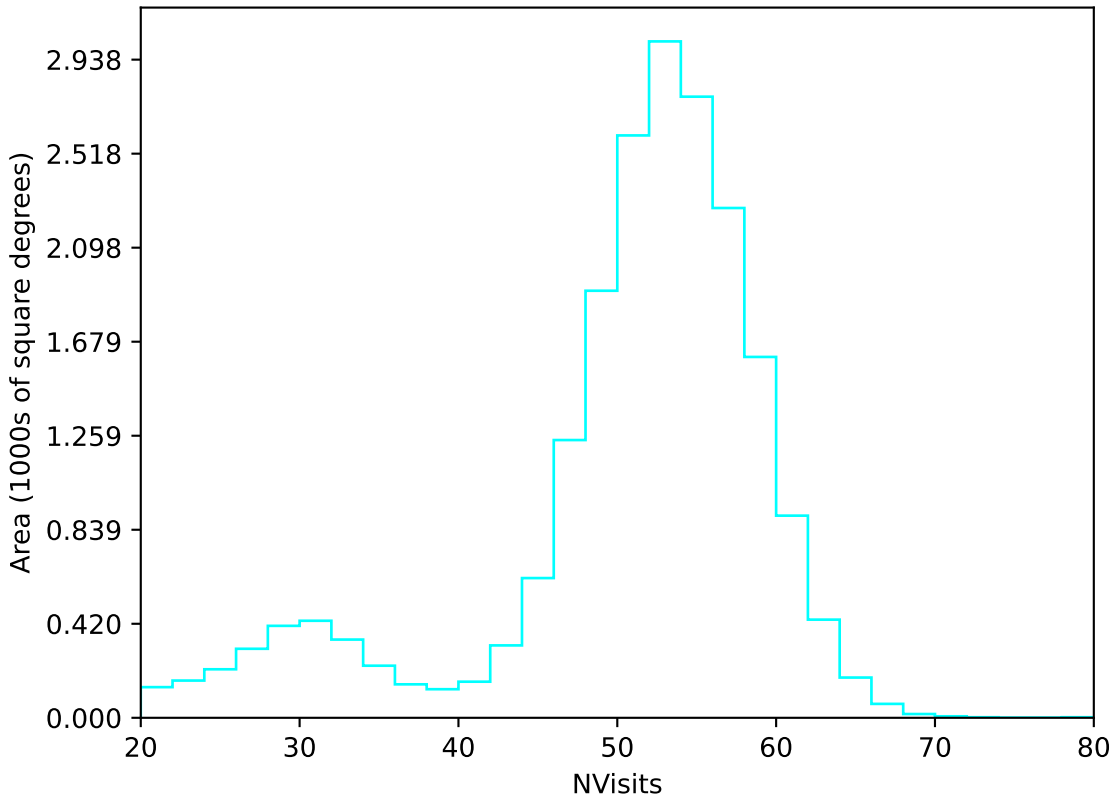
ddf_acor_sf20_lsf0_lsr0_v3.4_10yrs All sky u band: NVisits
