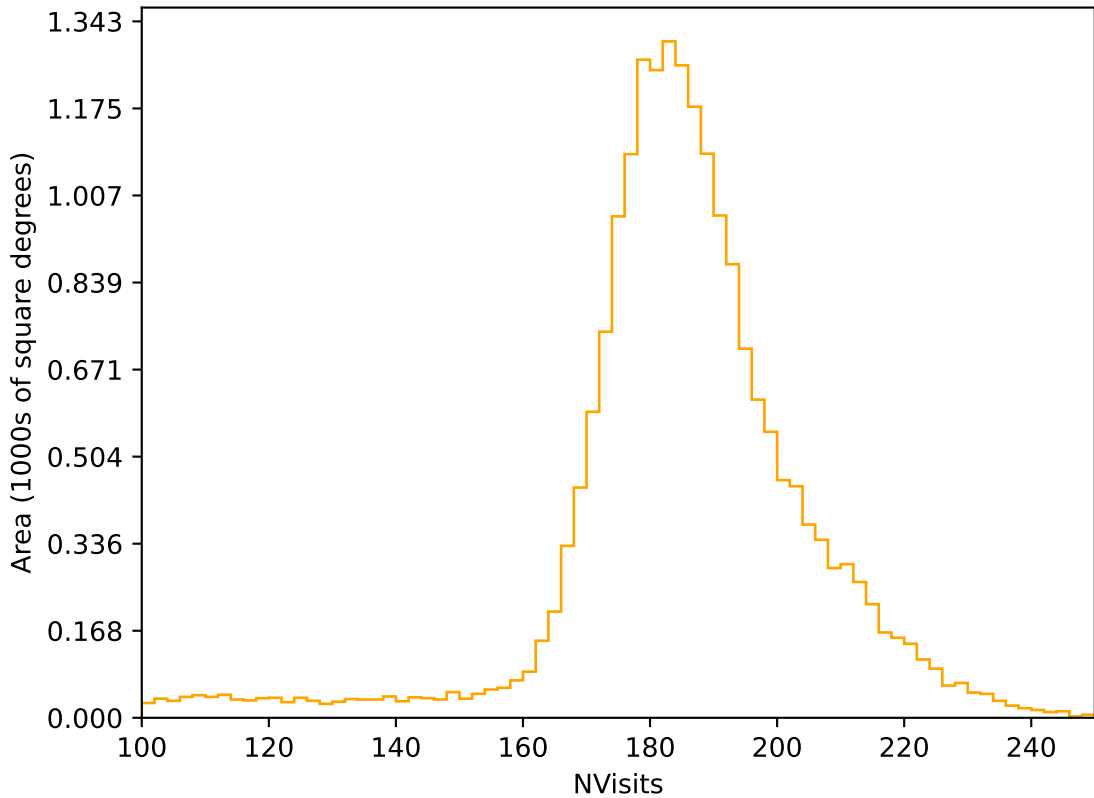
ddf_acor_sf20_lsf0_lsr0_v3.4_10yrs All sky r band: NVisits
