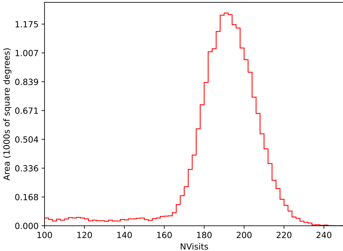
ddf_acor_sf20_ls0_lsr0_v3.4_10yrs All sky i band: NVisits
