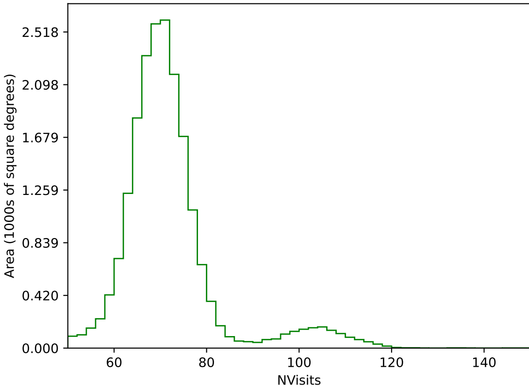
ddf_acor_sf20_lsf0_lsr0_v3.4_10yrs All sky g band: NVisits
