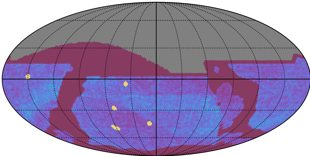
ddf_acor_sf20_lsf0_lsr0_v3.4_10yrs All sky all bands: NVisits
