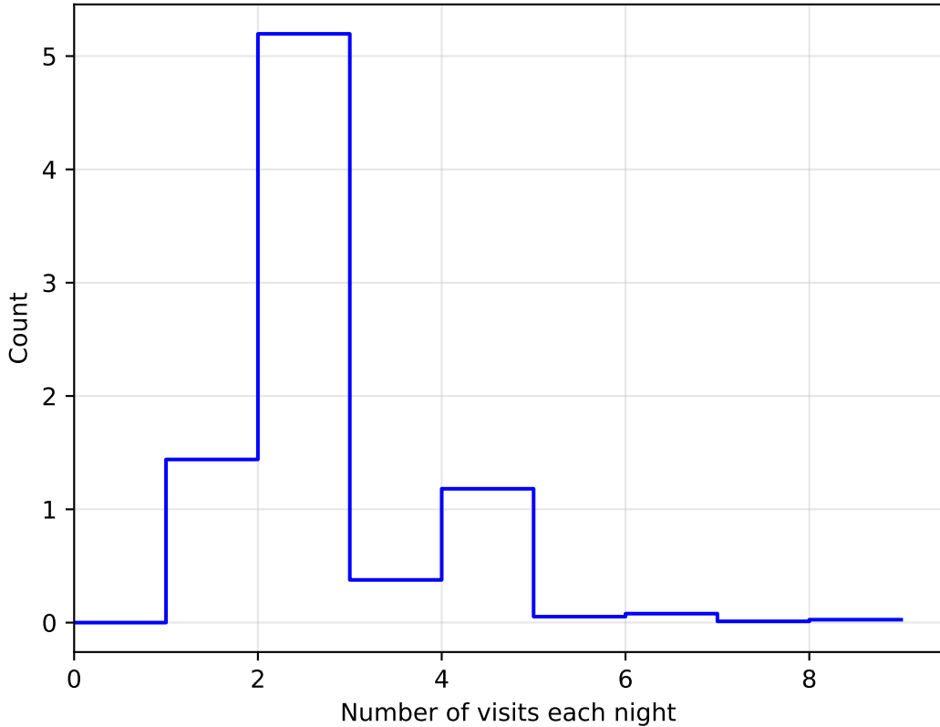
ddf_acor_sf20_lsf0_lsr0_v3.4_10yrs WFD: NVisitsPerNight 1e6
