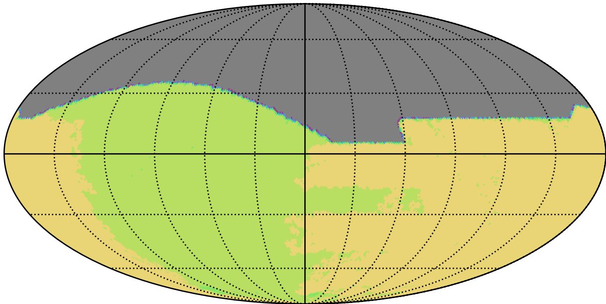
ddf_acor_sf20_lsf0_lsr0_v3.4_10yrs All sky all bands: NSeasons
