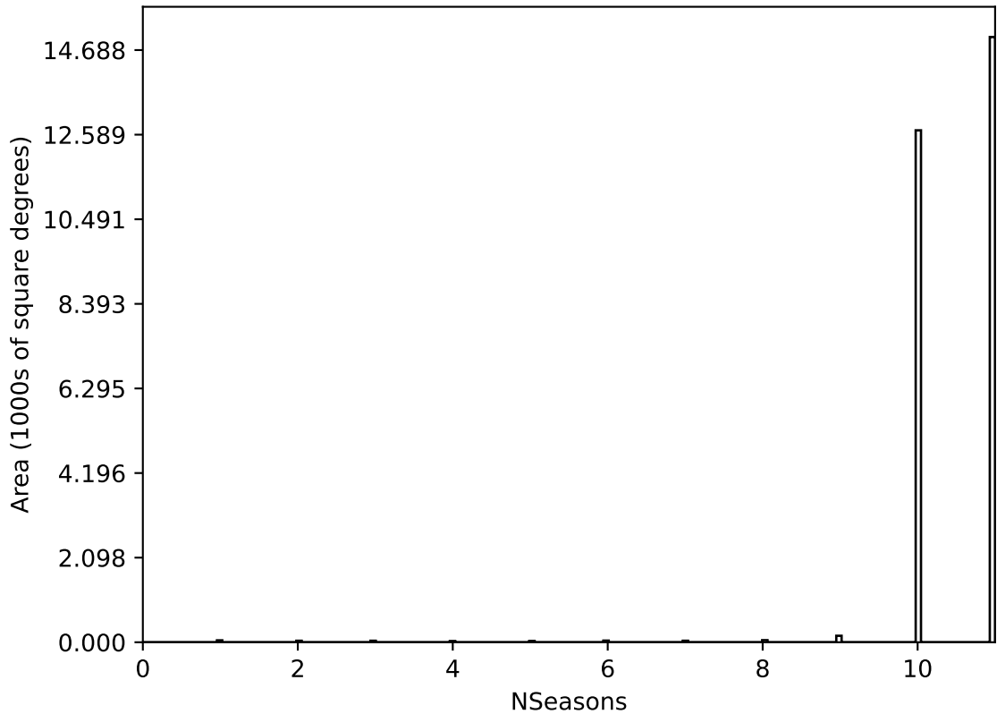
ddf_acor_sf20_lsf0_lsr0_v3.4_10yrs All sky all bands: NSeasons
