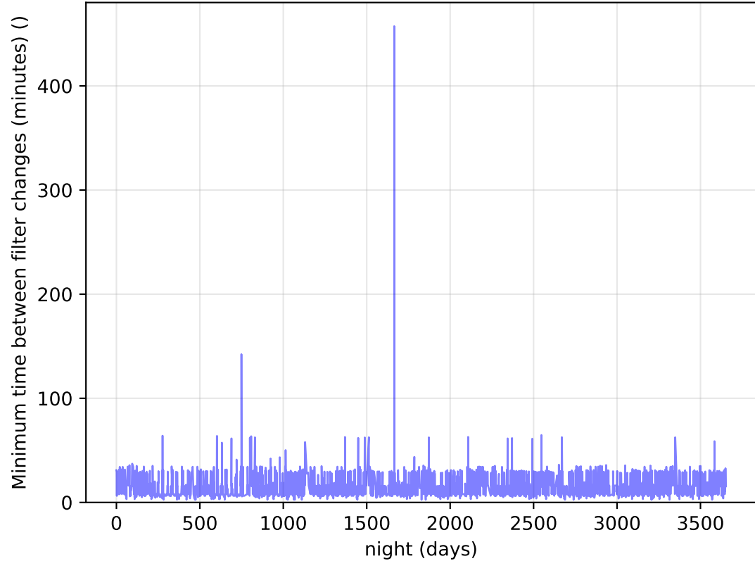
ddf_acor_sf20_Isf0_Isr0_v3.4_10yrs Per Night: Minimum time between filter changes (minutes)
