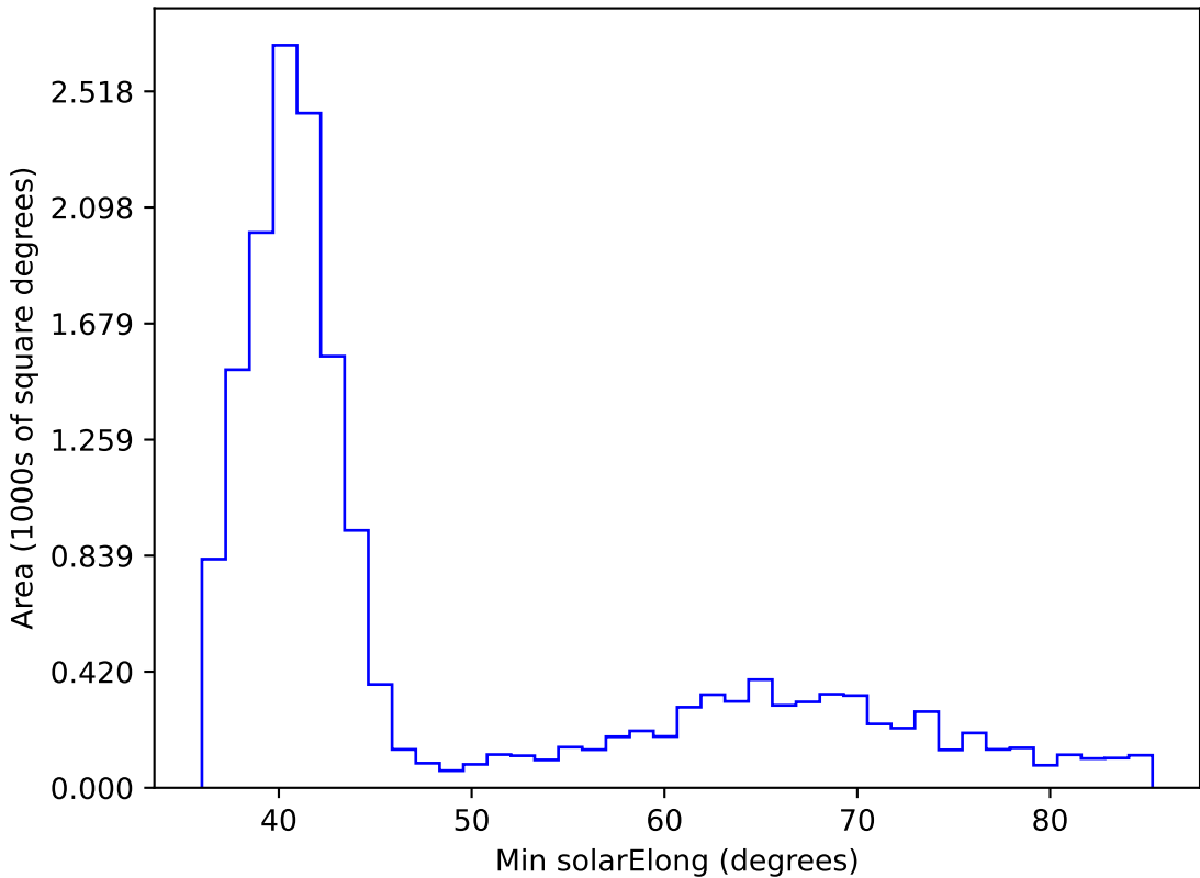
ddf_acor_sf20_lsf0_lsr0_v3.4_10yrs WFD z band: Min solarElong
