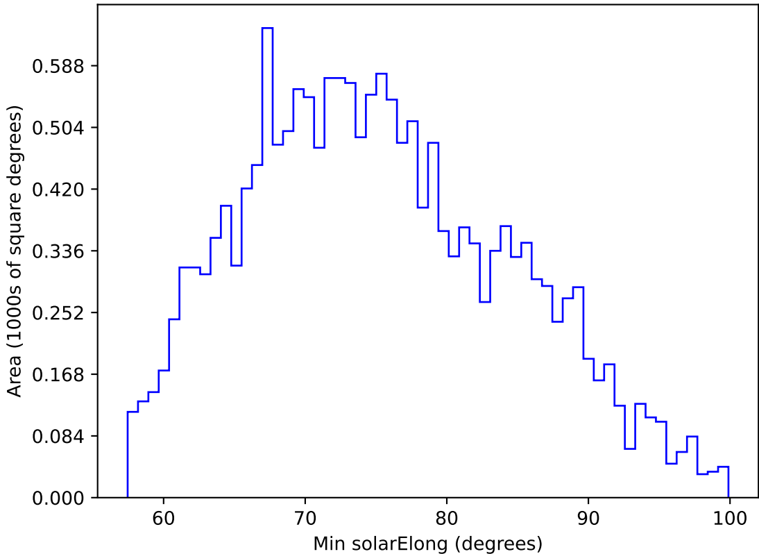
ddf_acor_sf20_ls0_lsr0_v3.4_10yrs WFD u band: Min solarElong
