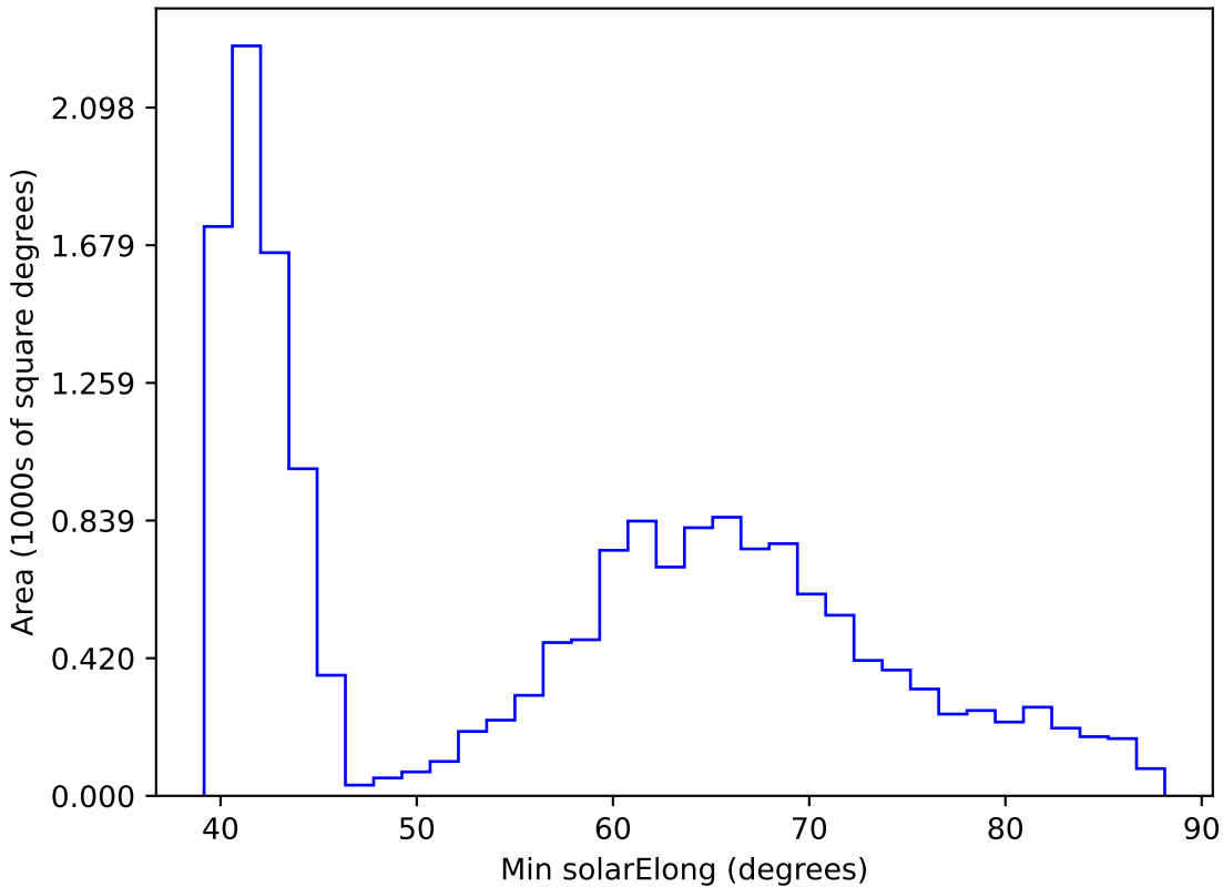
ddf_acor_sf20_lsf0_lsr0_v3.4_10yrs WFD r band: Min solarElong
