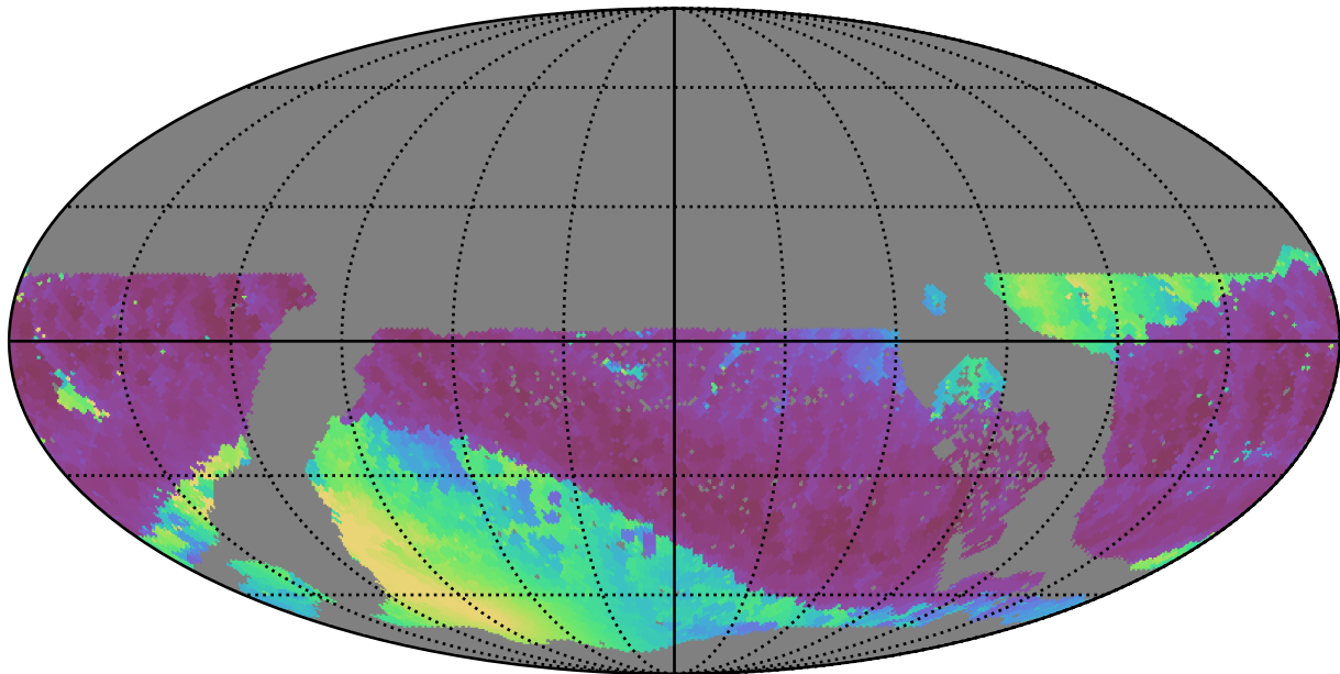
ddf_acor_sf20_lsf0_lsr0_v3.4_10yrs WFD i band: Min solarElong
