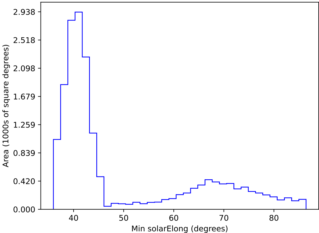
ddf_acor_sf20_lsf0_lsr0_v3.4_10yrs WFD i band: Min solarElong
