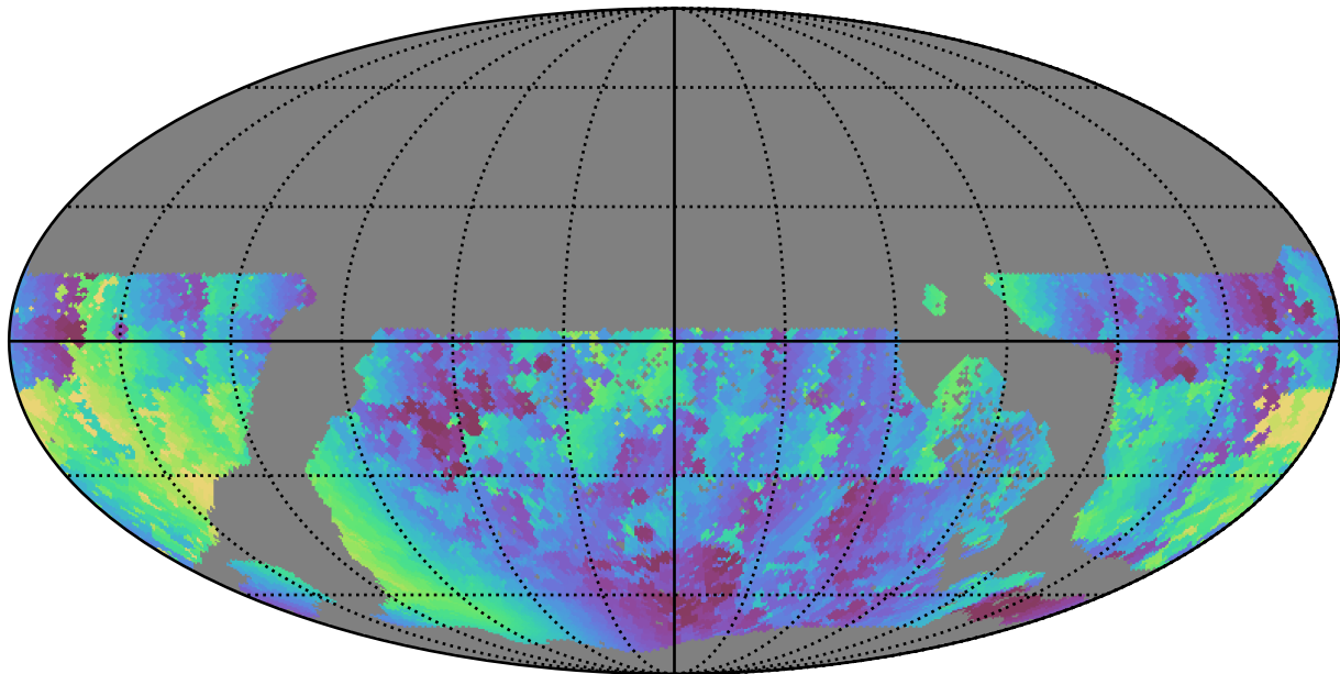
ddf_acor_sf20_lsf0_lsr0_v3.4_10yrs WFD g band: Min solarElong
