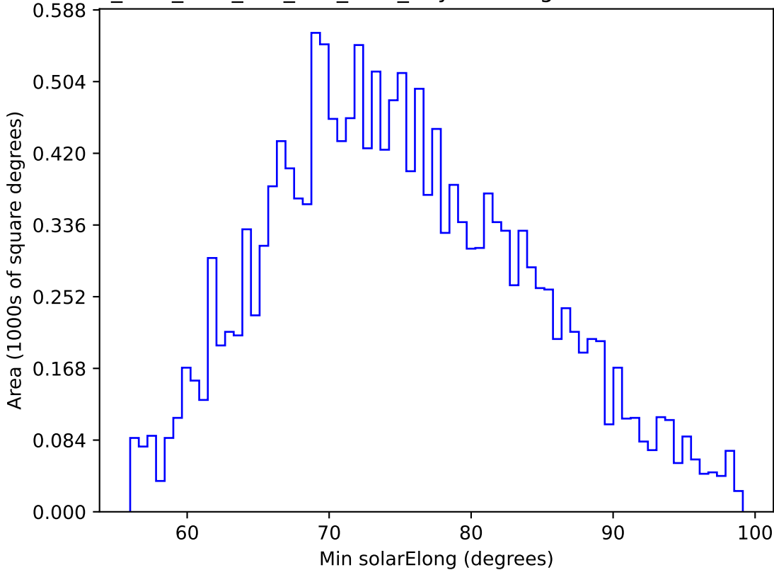
ddf_acor_sf20_lsf0_lsr0_v3.4_10yrs WFD g band: Min solarElong
