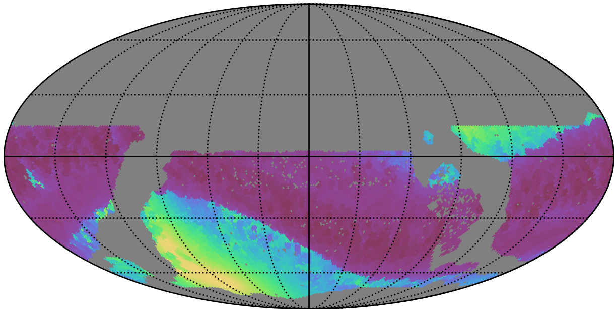
ddf_acor_sf20_lsf0_lsr0_v3.4_10yrs WFD all bands: Min solarElong
