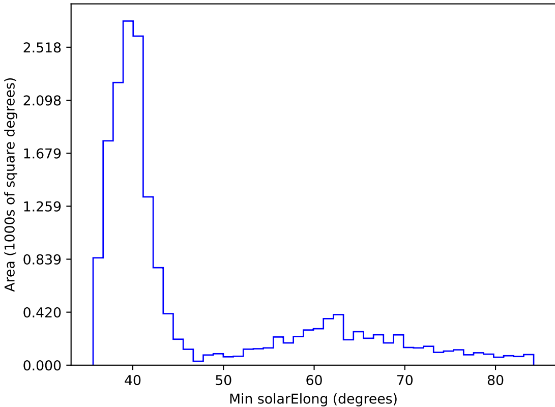
ddf_acor_sf20_lsf0_lsr0_v3.4_10yrs WFD all bands: Min solarElong
