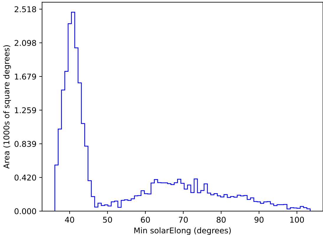
ddf_acor_sf20_lsf0_lsr0_v3.4_10yrs All sky z band: Min solarElong
