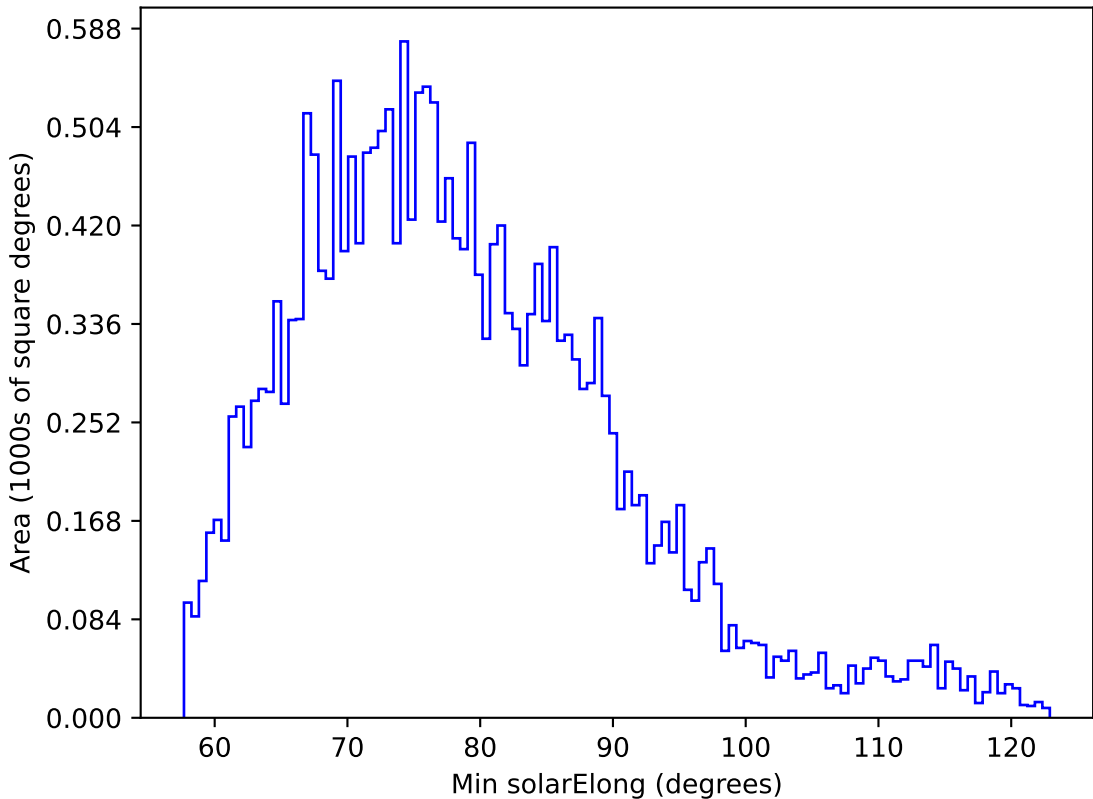
ddf_acor_sf20_lsf0_lsr0_v3.4_10yrs All sky u band: Min solarElong
