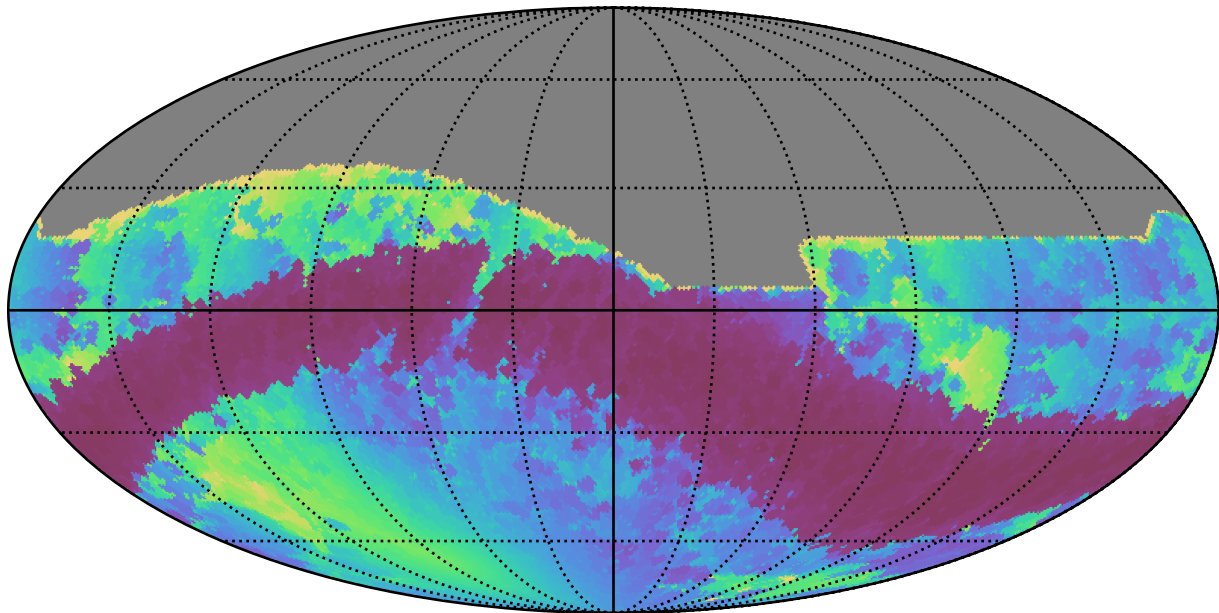
ddf_acor_sf20_lsf0_lsr0_v3.4_10yrs All sky r band: Min solarElong
